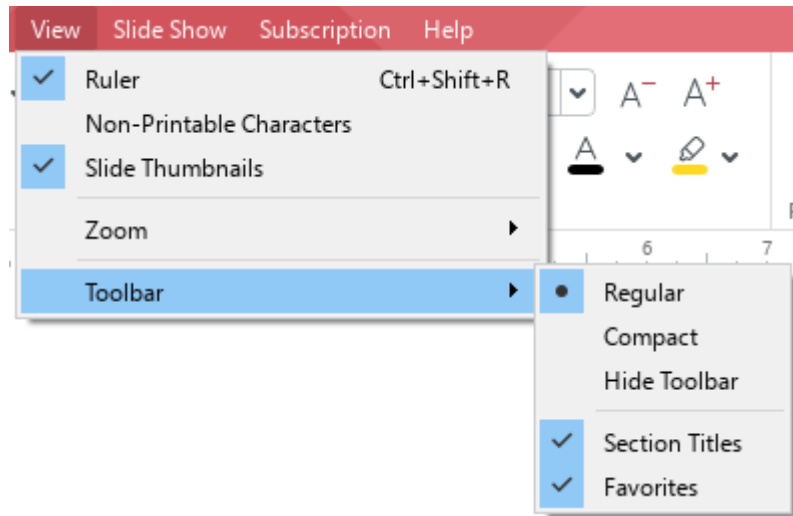
Figure 30. Toolbar sub-menu
