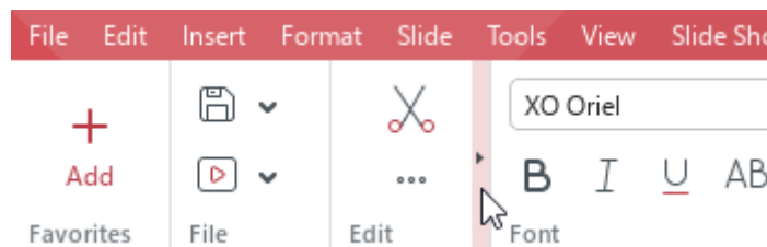
Figure 23. Expand button
