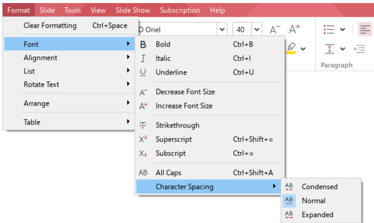
Figure 102. Format menu
