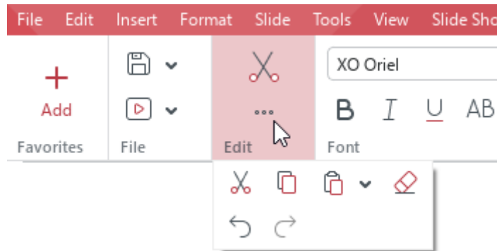
Figure 22. Section tools
