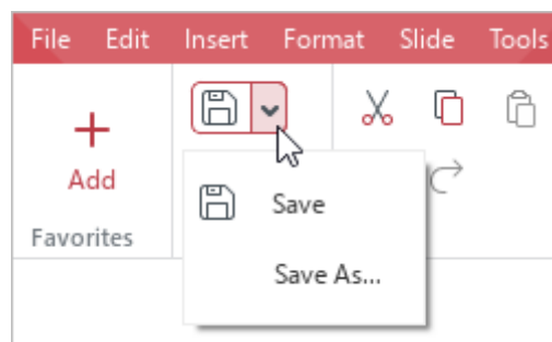
Figure 53. Save button
