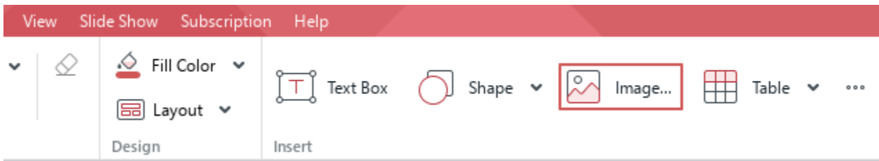
Figure 134. Image button
