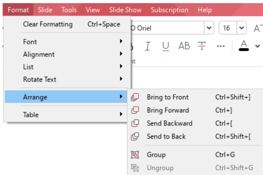
Figure 197. Format menu
