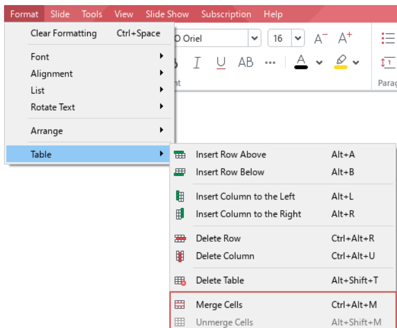
Figure 187. Format menu
