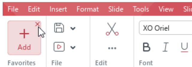
Figure 31. Favorites section
