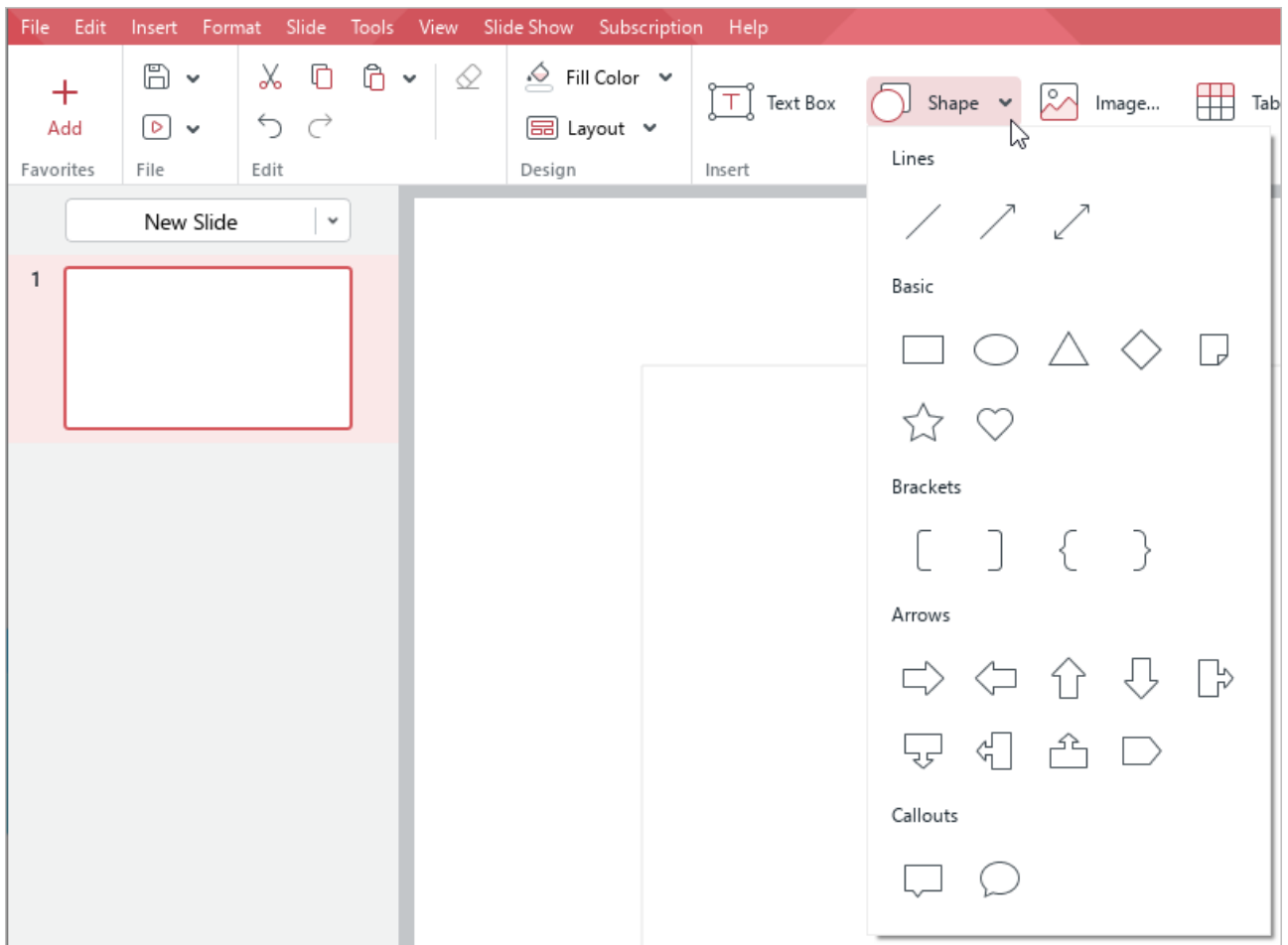
Figure 148. Shape button
