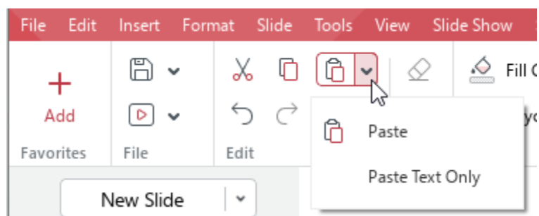
Figure 217. Paste button
