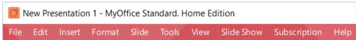
Figure 16. Command menu
