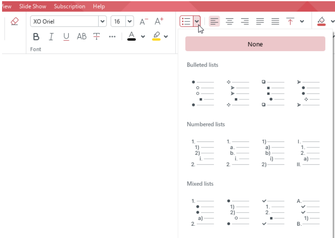
Figure 110. List button
