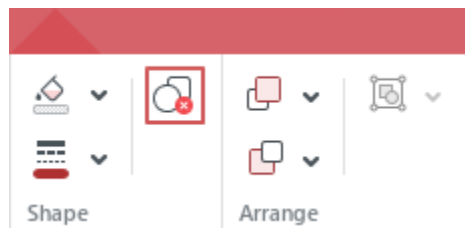
Figure 210. Delete button
