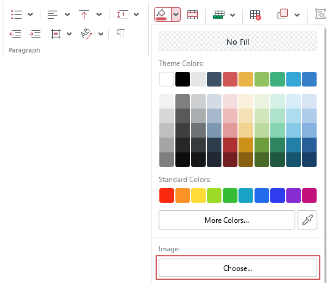
Figure 191. Choose button
