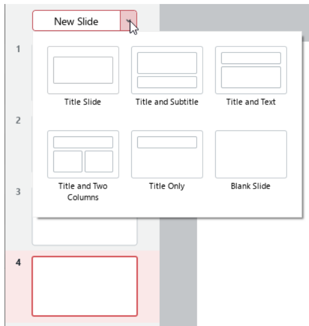
Figure 72. Slide layouts
