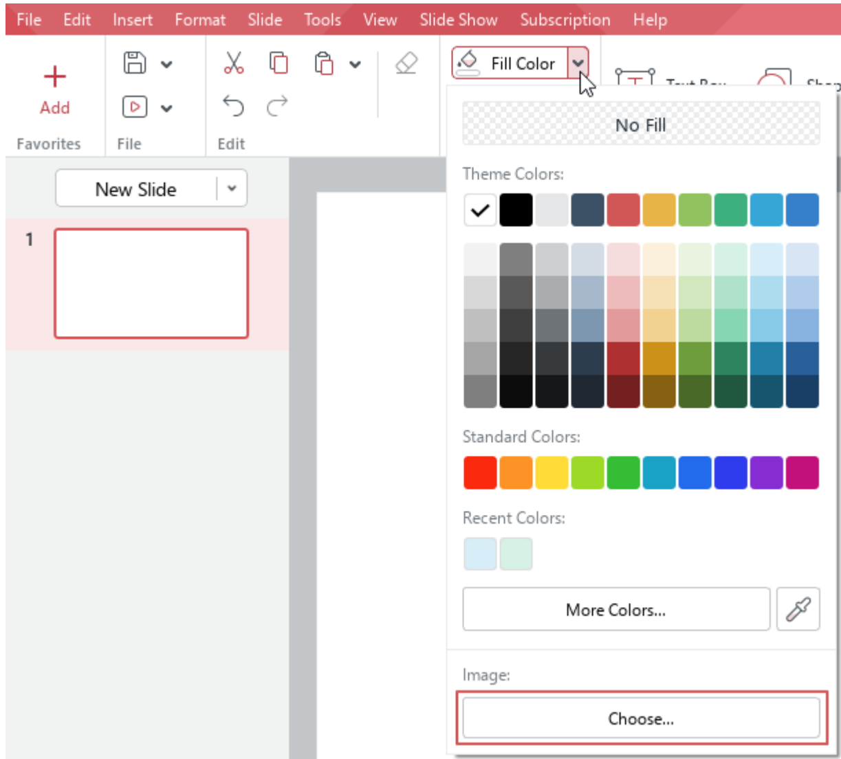
Figure 86. Choose button
