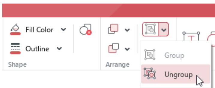
Figure 207. Ungroup command
