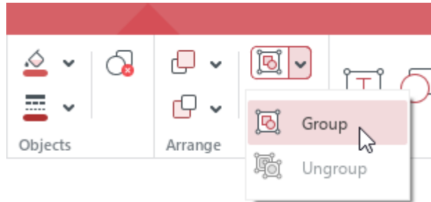
Figure 204. Group command
