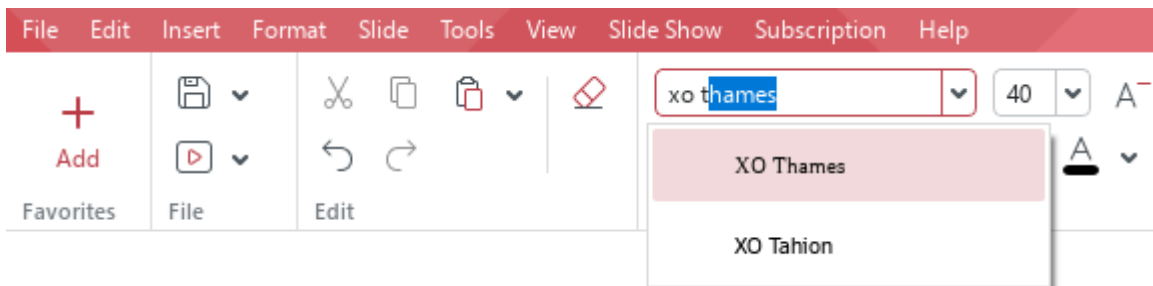
Figure 92. Font search
