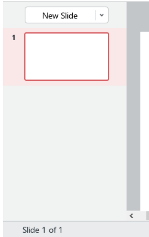
Figure 32. Slide bar
