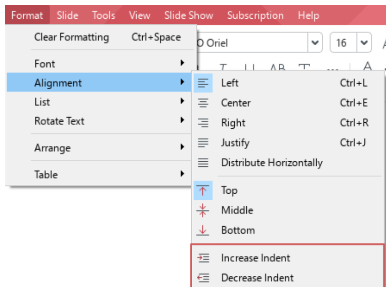
Figure 111. Format menu
