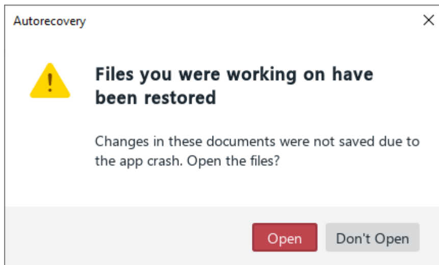
Figure 56. Dialog box
