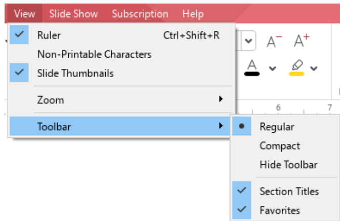
Figure 18. View menu
