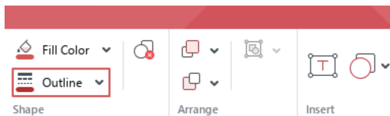
Figure 159. Outline button
