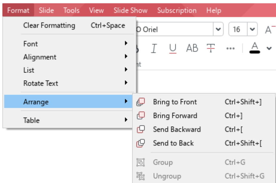
Figure 143. Format menu
