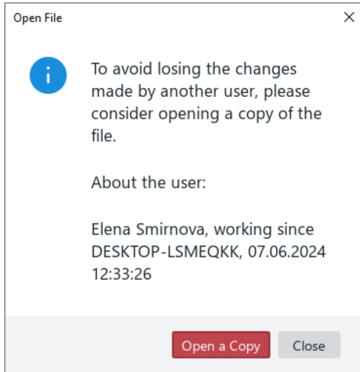
Figure 48. Dialog box
